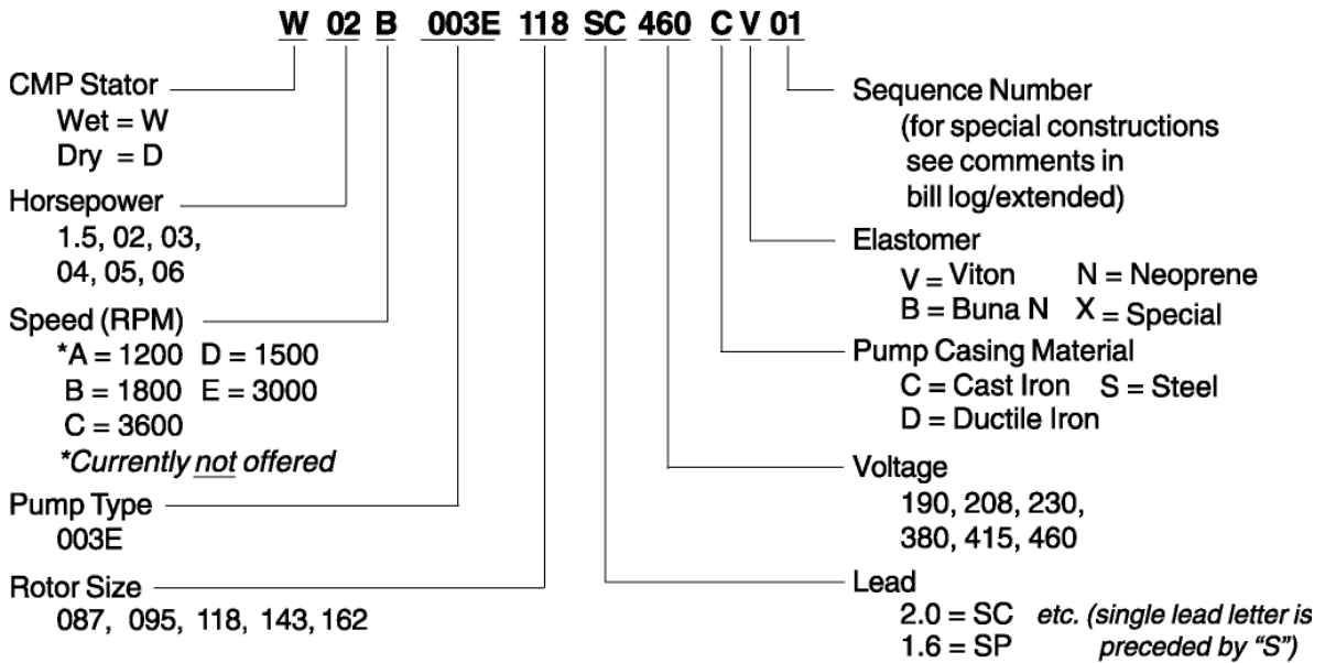
Figure 1 – Model Designation
