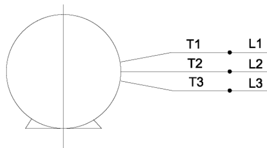
3 Phase-Single Voltage
